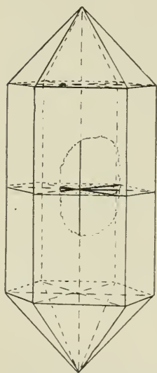
SAND-GRAIN WITH SECONDARY QUARTZ.
